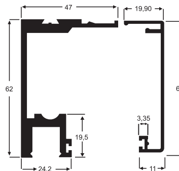
1041 1,192 Kg/m
